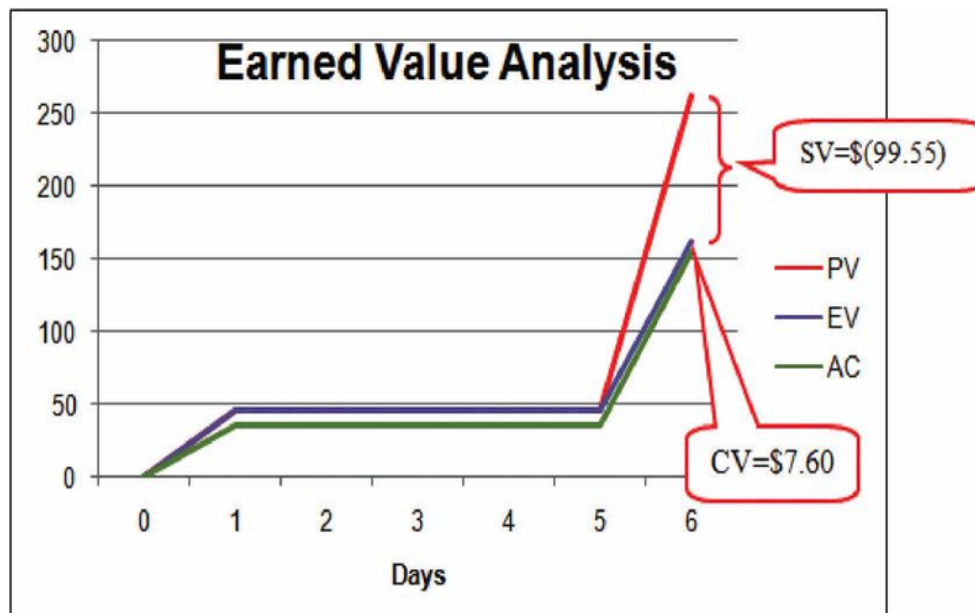
Figure 12.7 Schedule Variance and Cost Variance
