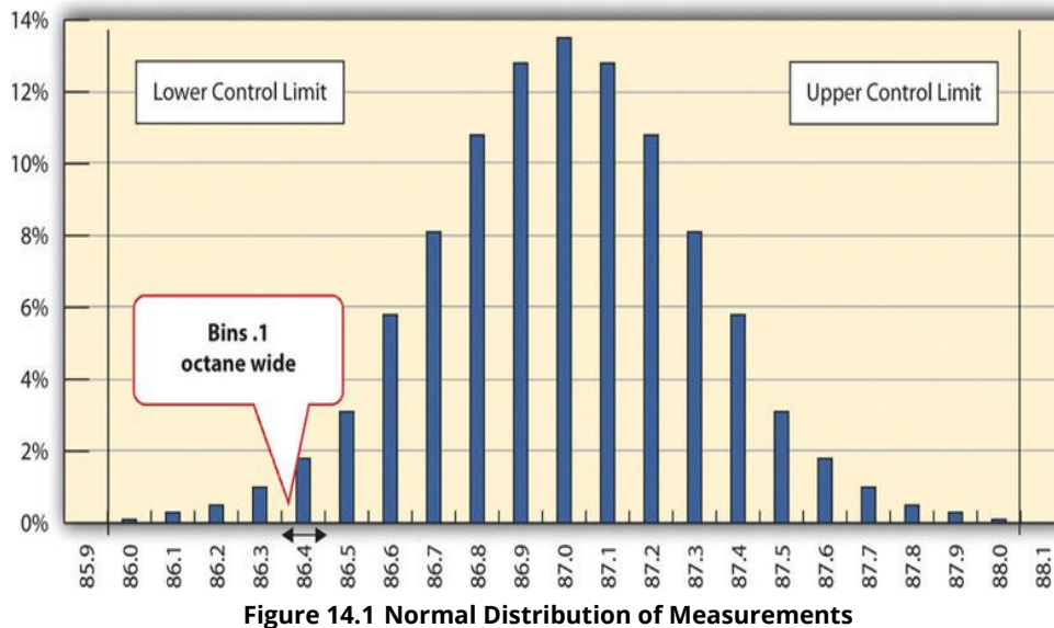
Figure 14.1 Normal Distribution of Measurements
