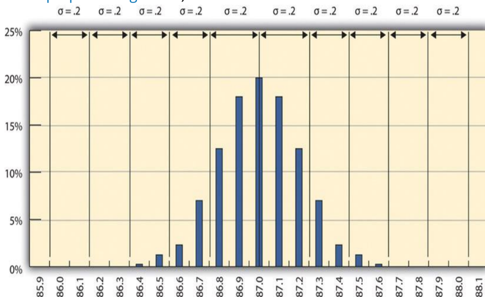
Figure 14.4 Smaller Standard Deviation
