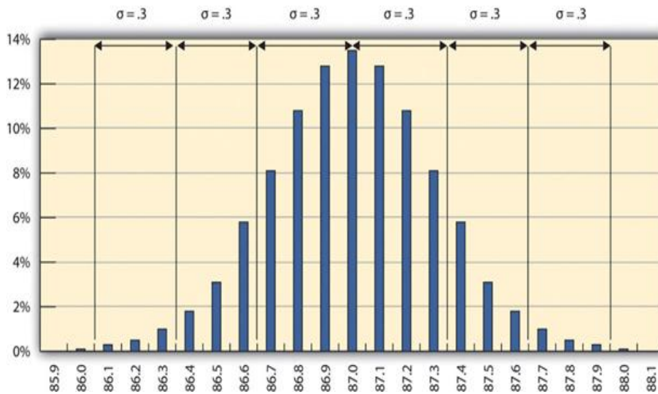
Figure 14.3 The 68-95-99.7 Rule
