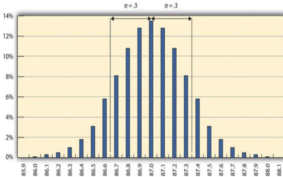
Figure 14.2 One Sigma Range Most of the measurements are within 0.3 octave of 87.
